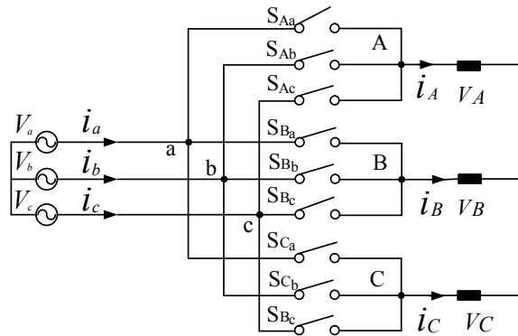
Figure.1 Topology of three-to-three-phase direct matrix converter
