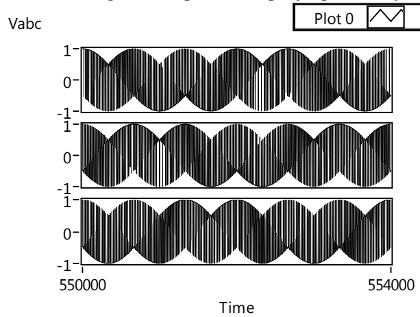
Figure.6 Phase voltages with input and output frequencies of 50 and 40 Hz
