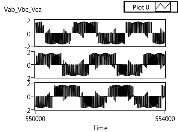
Figure.5 Line to line voltages with input and output frequencies of 50 and 60 Hz
