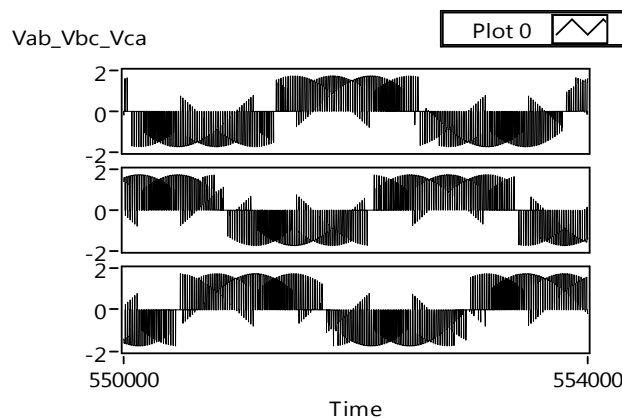
Figure.3 Line to line voltages with input and output frequencies of 50 and 40 Hz
