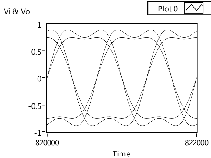
Figure.2. Envelope of Input and output voltages for 86.6 % voltage transfer ratio in three-to-three phase direct matrix converter
