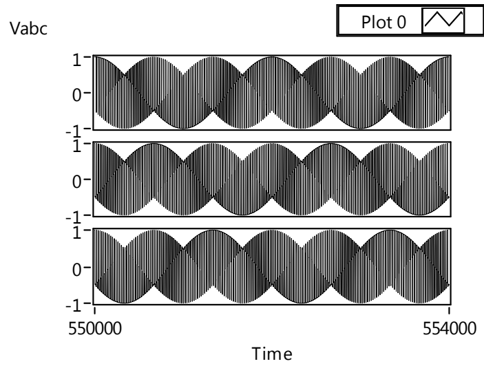
Figure.7 Phase voltages with input and output frequencies of 50 and 50 Hz
