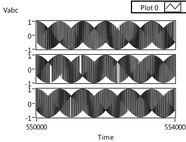
Figure.8 Phase voltages with input and output frequencies of 50 and 60 Hz
