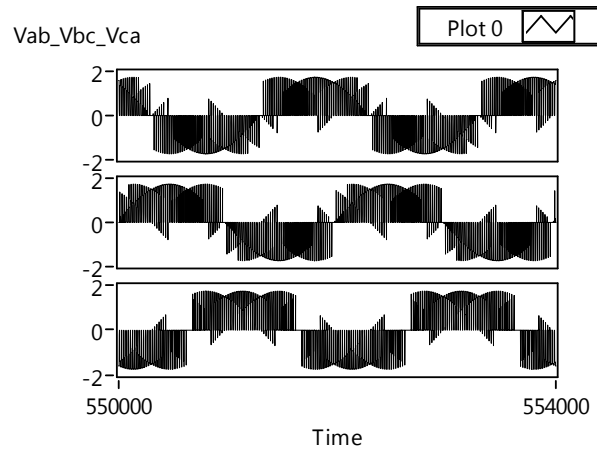
Figure.4 Line to line voltages with input and output frequencies of 50 and 50 Hz
